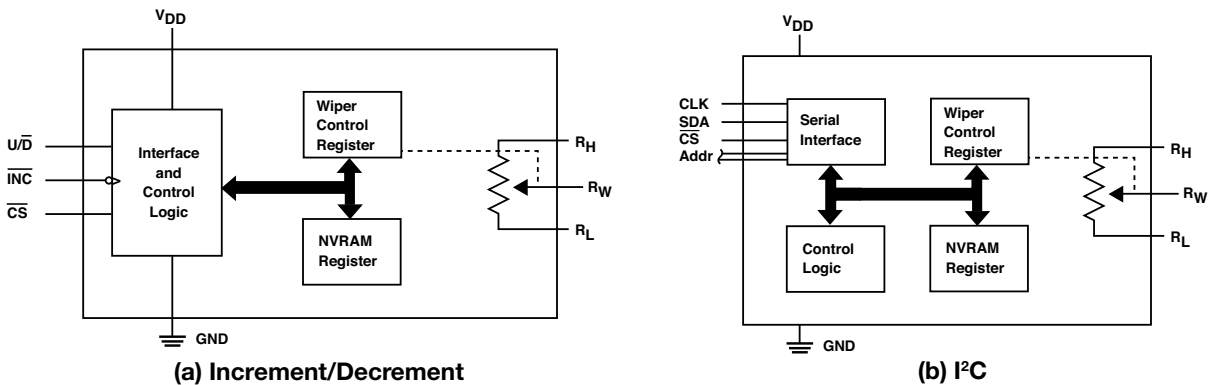
Figure 3. Serial Interfaces
