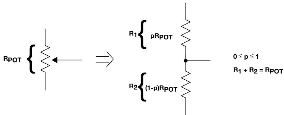
Figure 7. Mathematical Model of the Pot Resistances
