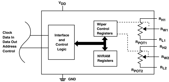
Figure 2. Control of Electronic Potentiometers
