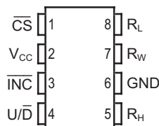
TSSOP 8 Lead (Y)
