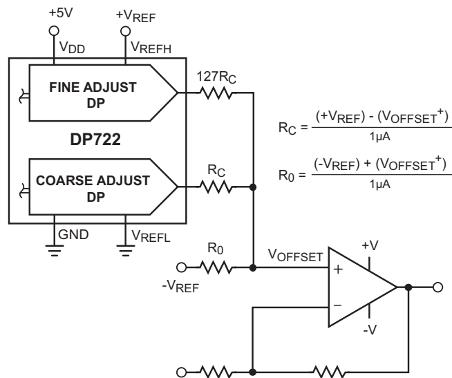
Coarse-Fine Offset Control by Averaging DP Outputs for Dual Power Supply Systems
