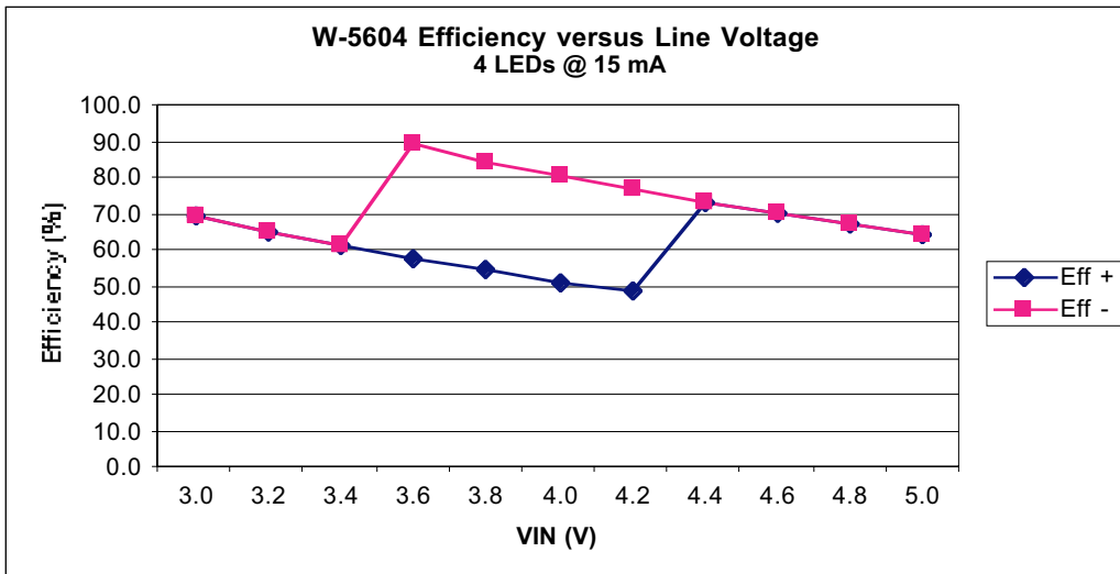
Figure 8. W-5604 Efficiency versus Line Voltage
