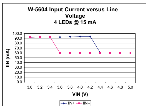
Figure 5. Input Current versus Line Voltage
