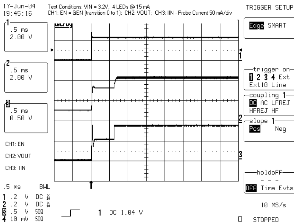
Figure 11. W-5604 Wake-Up from Shutdown Mode (VIN = 3.2V)
