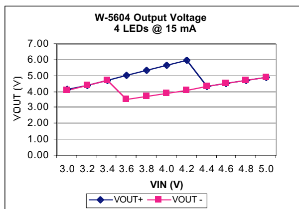
Figure 6. Output Voltage versus Line Voltage
