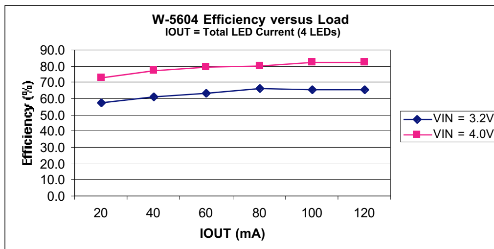
Figure 9. W-5604 Efficiency versus Load
