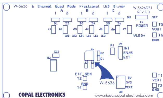
Figure 2. W-5636DB1 Board
