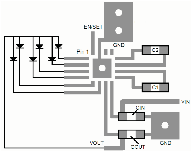
Figure 5. Recommended Layout
