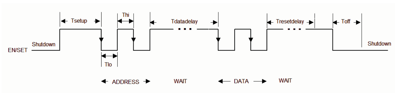
Figure 1. EN/SET One Wire Addressable Timing Diagram
