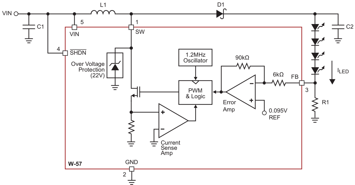
Figure 2. W-57 Block Diagram
