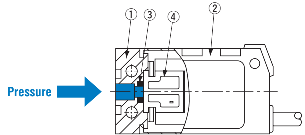
INTERNAL STRUCTURE (M5 female screw)
